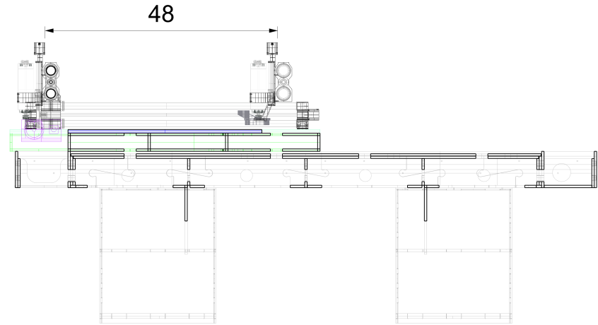
RIGHT SECTION NTS
